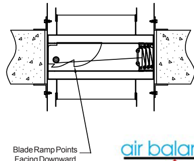
Type C, Field Sleeve, Horizontal
